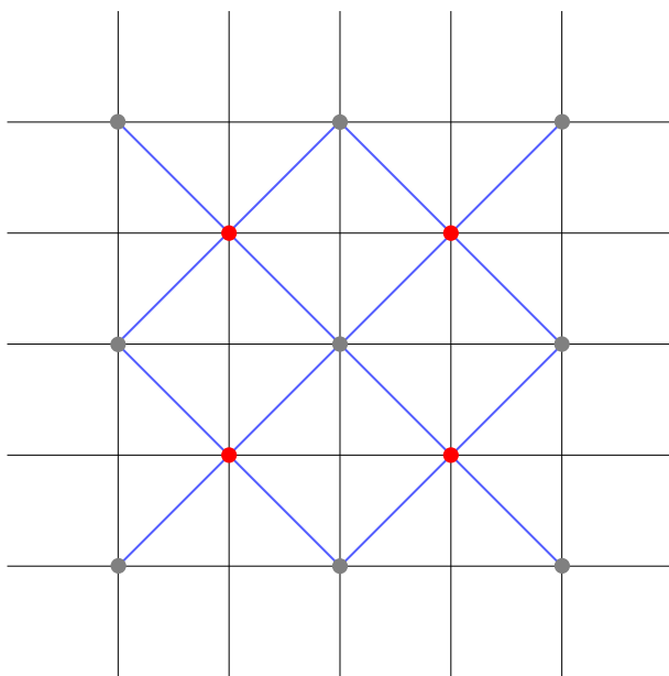
Figure 349: How the diamond-square algorithm works (4/5)
